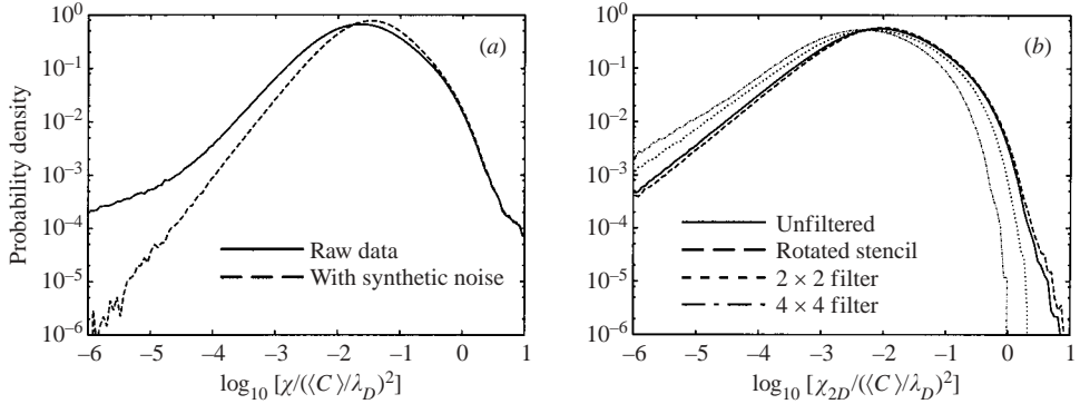
FIGURE 7. The effects of measurement noise and spatial resolution on the PDFs of the scalar dissipation rate, conditioned on |x/\delta| \leq 0.28 . (a) PDFs of the logarithm of \chi for the raw data, and for the data as contaminated with synthetic random noise. (b) PDFs of the logarithm of \chi_{2D} for the raw data, for the raw data using the rotated differencing stencil, and for the data after 2 \times 2 and 4 \times 4 box filtering.
