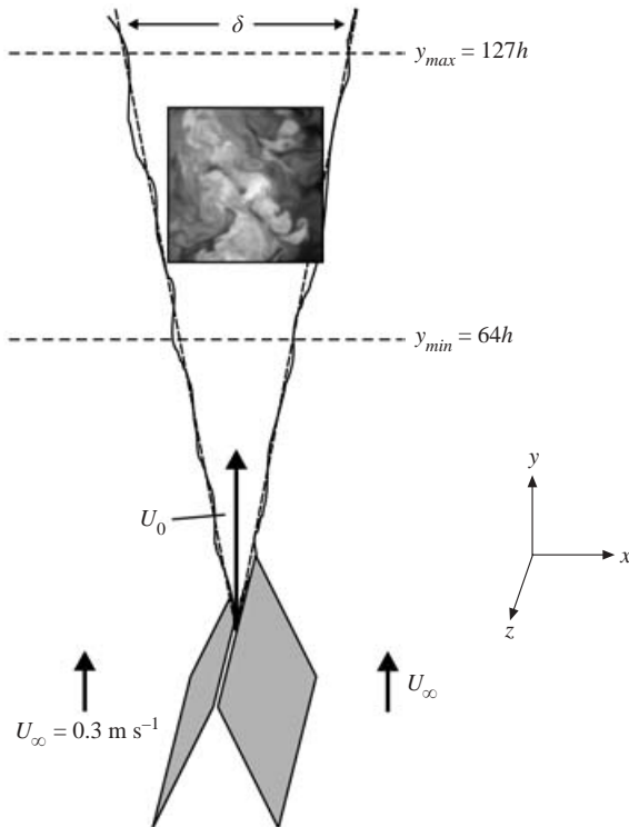
FIGURE 1. Sketch of the co-flowing planar turbulent jet, with a sample data plane from the set labelled f2 in table 1. Also indicated are the full width at 5% of maximum of the mean velocity profile, and the upstream and downstream limits of the measurement area for the full set of data.
