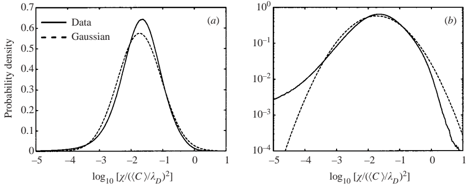
FIGURE 5. The PDF of the logarithm of the scalar dissipation rate, \chi , with (a) linear and (b) logarithmic y-axis, compared with the Gaussian distribution having the same first two moments. The mean value of \chi is indicated. The \chi distribution shows a small negative skewness.
