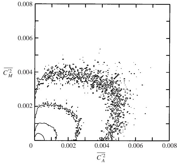
FIGURE 14. The joint PDF of the actual subgrid scalar variance, \overline{C_A^2} , and the scalar variance estimated by the gradient-based model, \overline{C_M^2} , with grid filter size \overline{\Delta} = 8 . The contour scale is logarithmic, with adjacent contours representing a magnitude ratio of 5.
